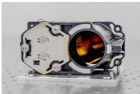
Fig. 2: The telescope developed by researchers in Jena and Freiburg will measure the Earth's water cycle in the future. © Fraunhofer IOF
